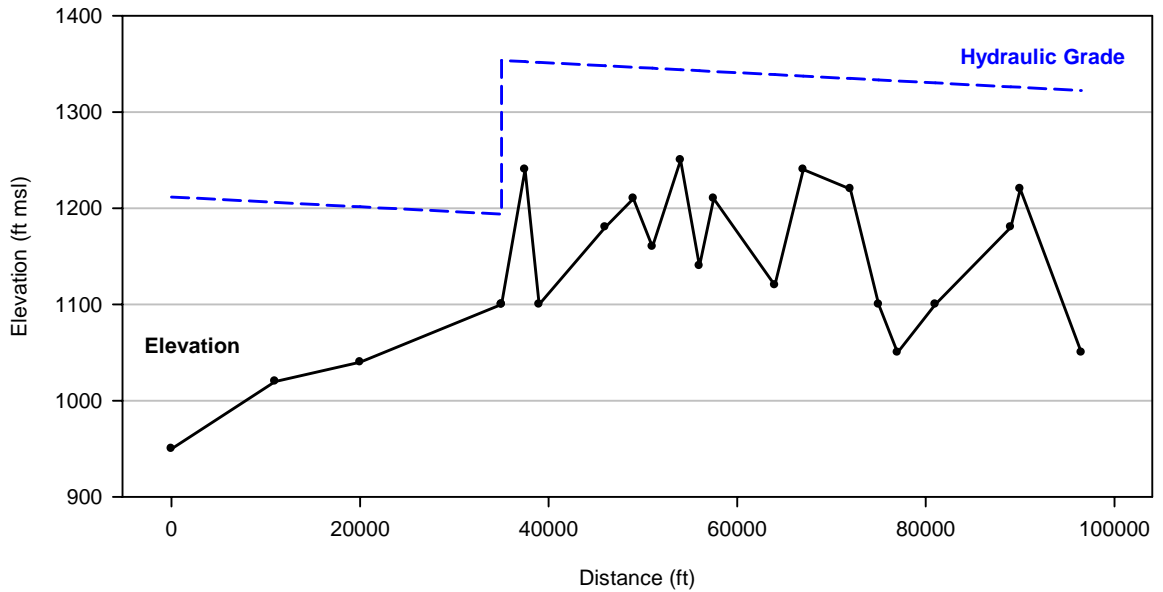
Figure C-24: Profile for P-10b (Indian Creek to Dry Frio Type 2).
