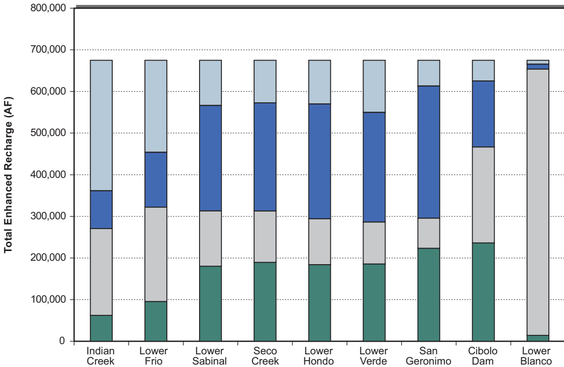
Figure 4-3 Results of 25,000 AFY Annual Recharge
