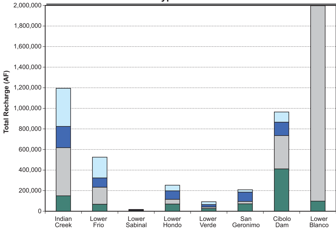
Figure 6-6 Total Yield From Type 2 Enhanced Recharge (Maximum Available Source Water)
