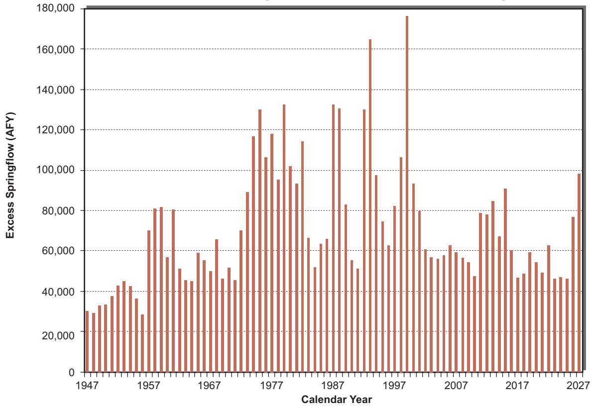
Excess Springflow With Enhanced Pumping
