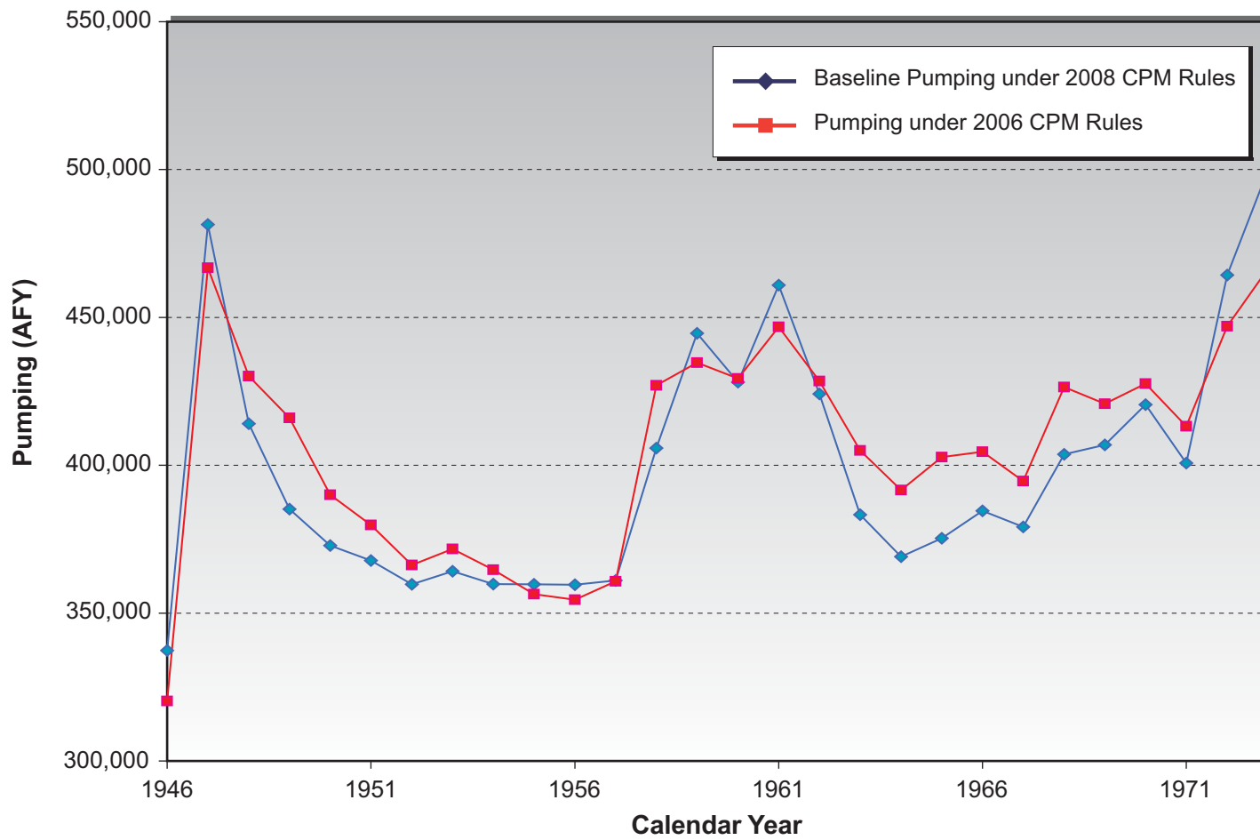
December 2008 Figure 3-1 Pumping Totals under CPM Rules TODD ENGINEERS Alameda, California
