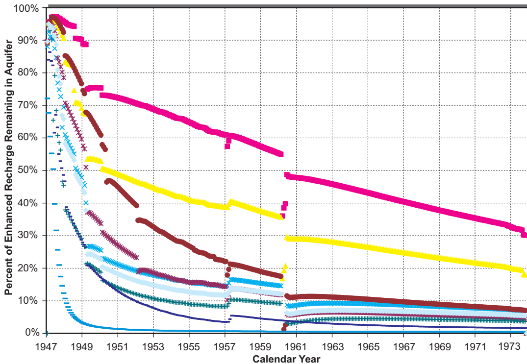
Recharge Slug in 1947 - 25,000 AF
