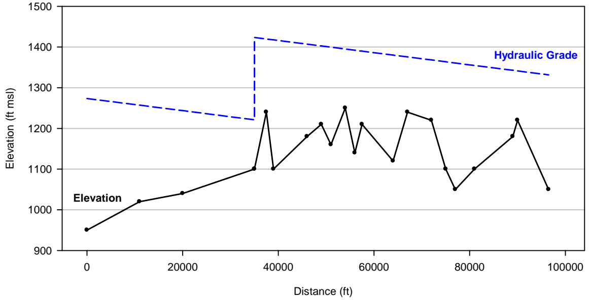
Figure C-23: Profile for P-10a (Indian Creek to Dry Frio Type 2).
